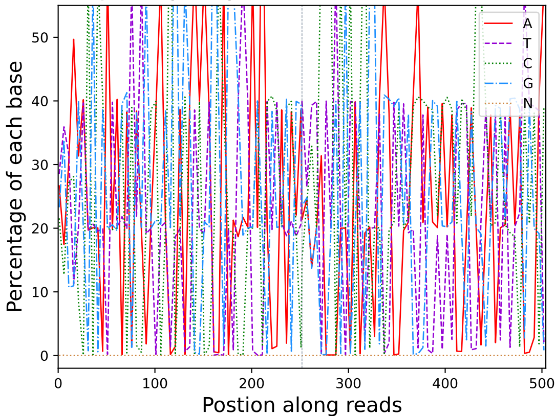
Base percentage along reads (R10124)
